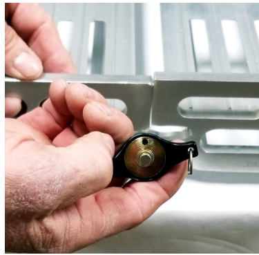
Connect sections to make ramps without tools Push button—Insert pin—release button—securely locks
